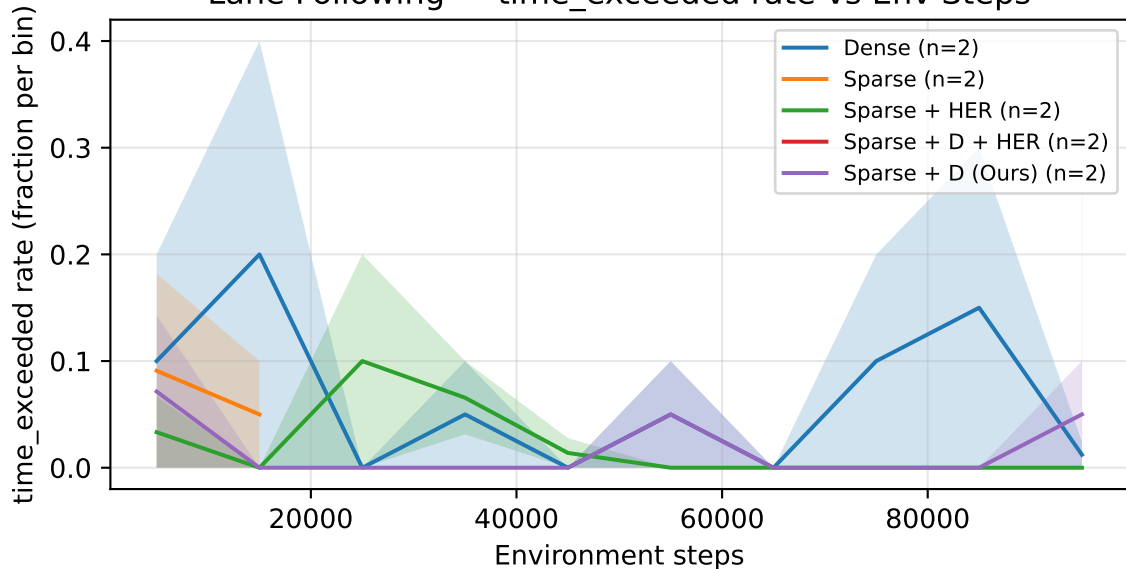
Lane Following — time_exceeded rate vs Env Steps
