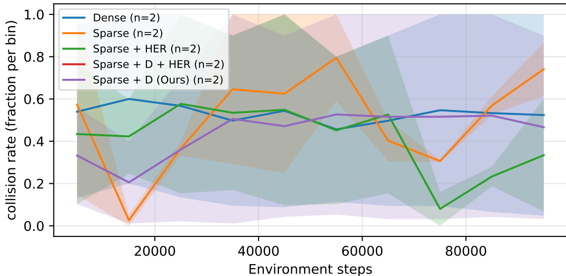
Overtaking — collision rate vs Env Steps
