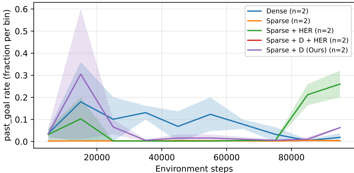
Overtaking — past_goal rate vs Env Steps
