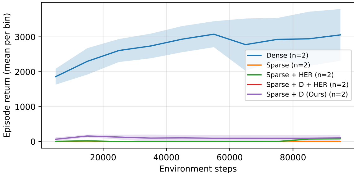
Overtaking — Return vs Env Steps
