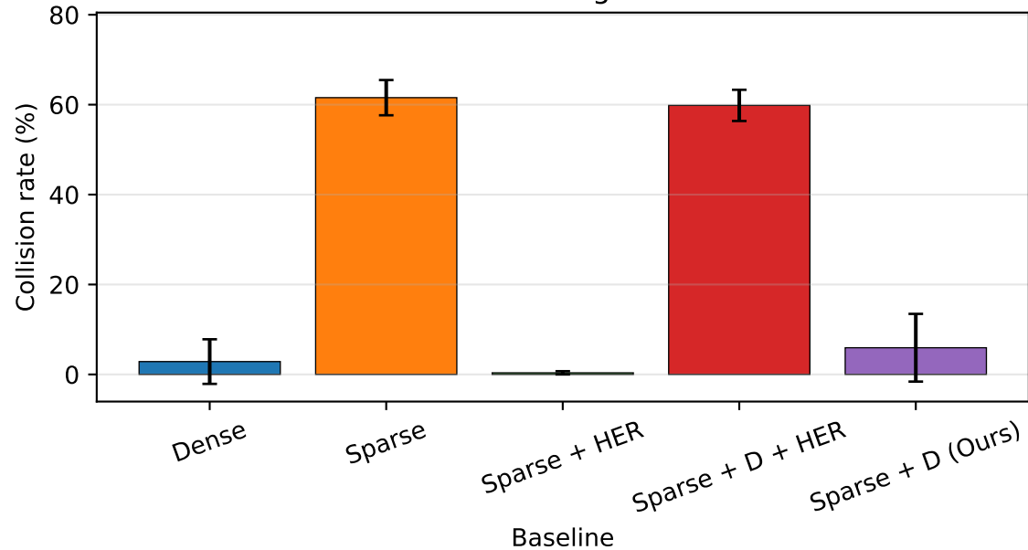
Lane Following — Seen
