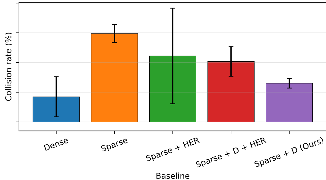
Lane Following — Unseen
