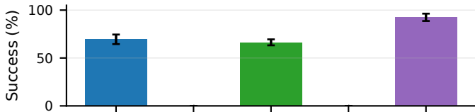
Lane-following — Unseen
