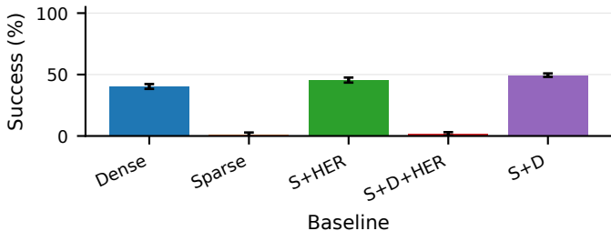
Lane-following — Unseen
