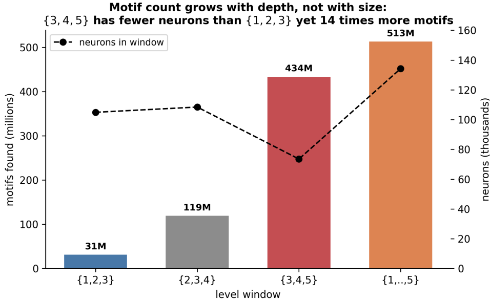
Figure 7: Number of bow-tie motifs found in each level window, shown as bars against the left axis, together with the number of neurons the window contains, shown as a dashed line against the right axis. The two do not track each other: window \{3, 4, 5\} contains fewer neurons than \{1, 2, 3\} yet yields fourteen times as many motifs.
