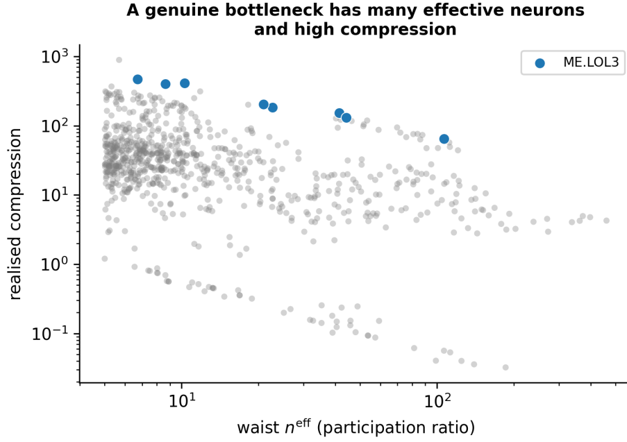
Figure 16: Realised compression against the effective number of waist neurons for window \{3, 4, 5\} , with the ME.LO_L3 family highlighted. Points at the far left achieve high compression through a single active neuron and are precisely the artefacts that the participation ratio is designed to expose. A genuine bottleneck lies towards the upper right, having both many effective neurons and high compression.
