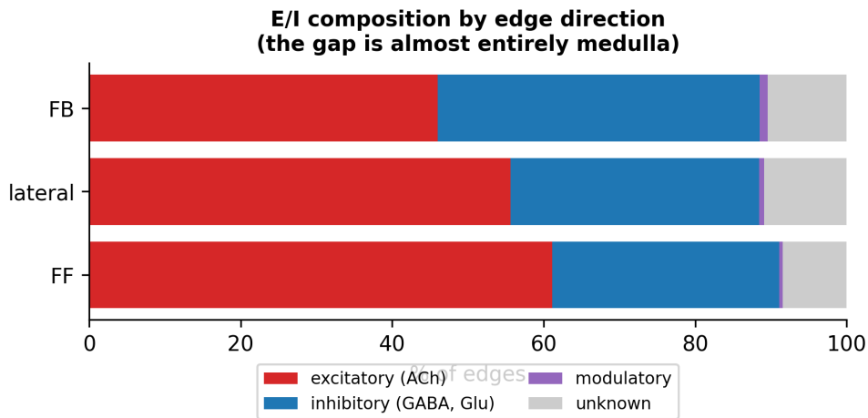
Figure 18: Excitatory and inhibitory composition of edges by direction. Feed-forward edges are more excitatory than feedback ones, but the difference is almost entirely attributable to the medulla. This figure concerns edges; the waist-level comparison that follows, which is the hypothesis actually under test, does not survive replication.
