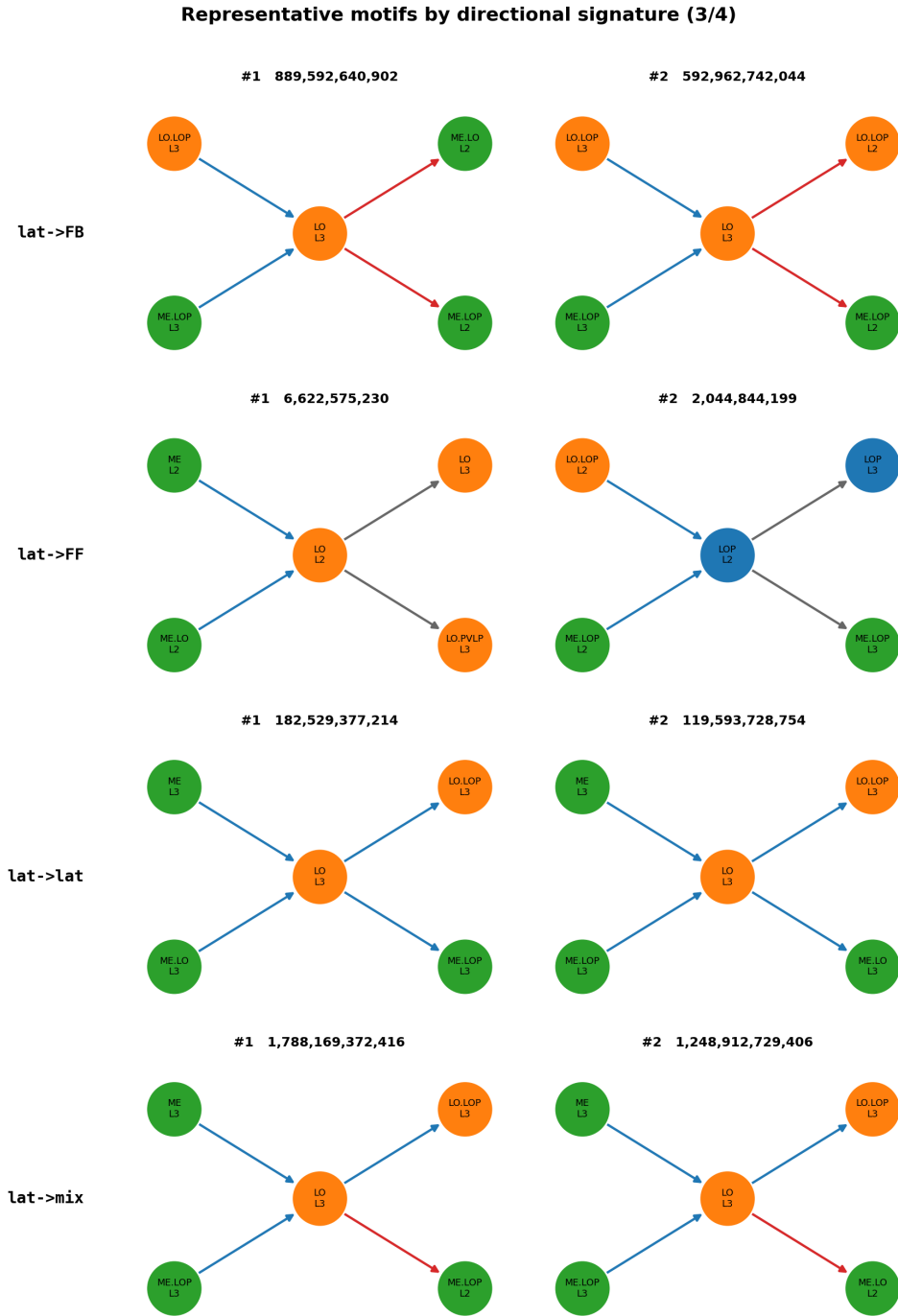
Figure 13: Representative motifs, signatures nine to twelve, with conventions as in Figure 11.
