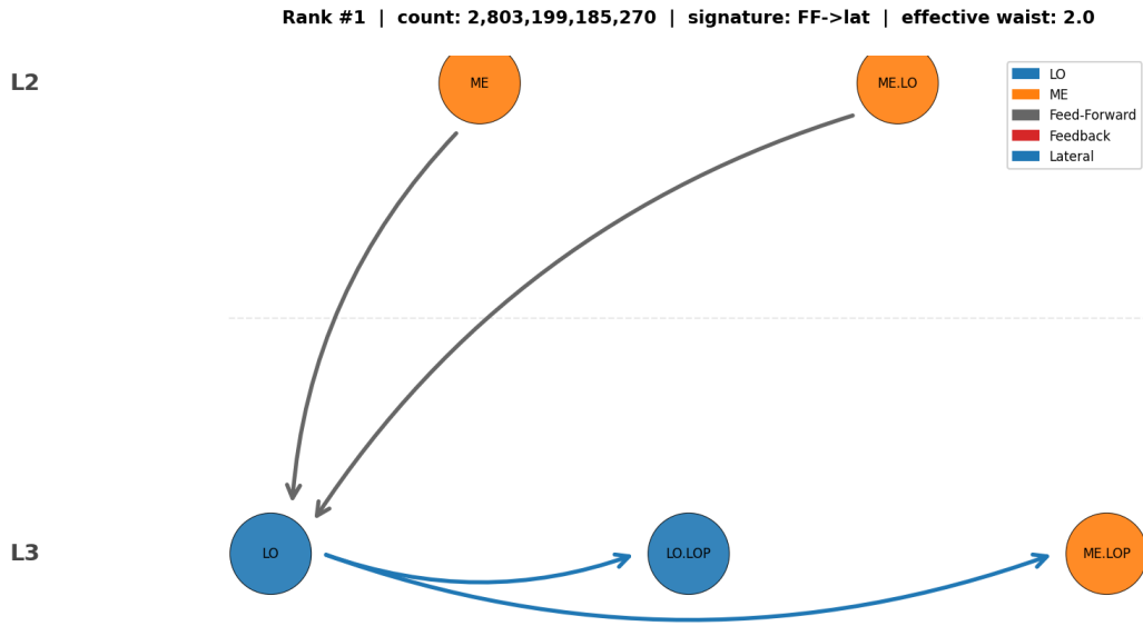
Figure 10: The single most frequent bow-tie motif of window \{1, 2, 3\} , with 2.80 \times 10^{12} instances and signature FF->lat . Two medulla groups at level 2 converge onto the lobula at level 3, which then distributes laterally within level 3. Grey edges are feed-forward and blue edges lateral. The pattern is a compact illustration of the general finding: the dominant structures combine a feed-forward entry with a lateral spread rather than being purely feed-forward.
