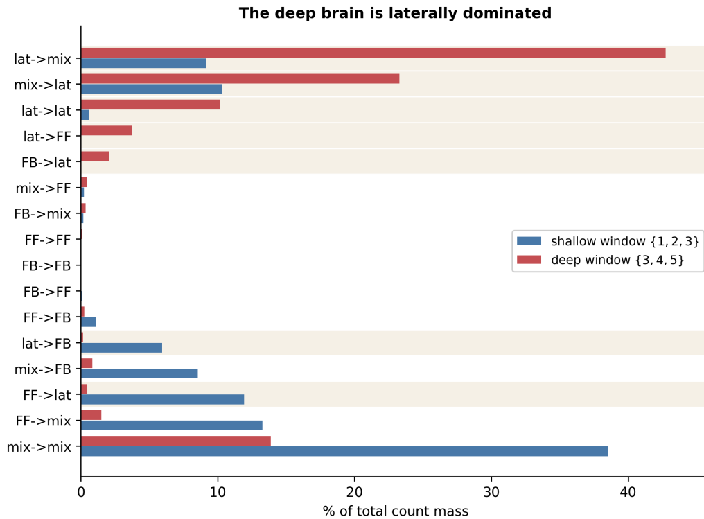
Figure 9: Share of total count mass by directional signature in the shallow and deep windows, sorted by the size of the shift between them. Shaded rows are signatures containing a purely lateral branch, and they gain almost exactly what the others lose. lat->mix alone rises from 9.2% to 42.7%.
