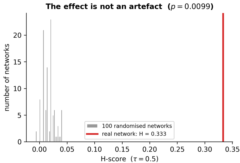
Figure 6: Distribution of the hourglass score over randomised networks, against the observed value. The observed score falls well outside the null distribution, establishing that the concentration of flow is not a by-product of the degree sequence alone.
