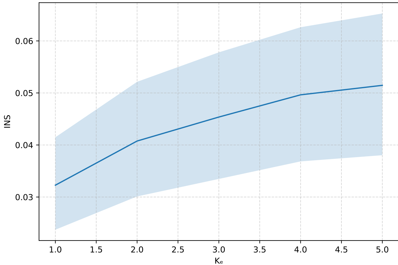
INS with 95% CI — LIME
