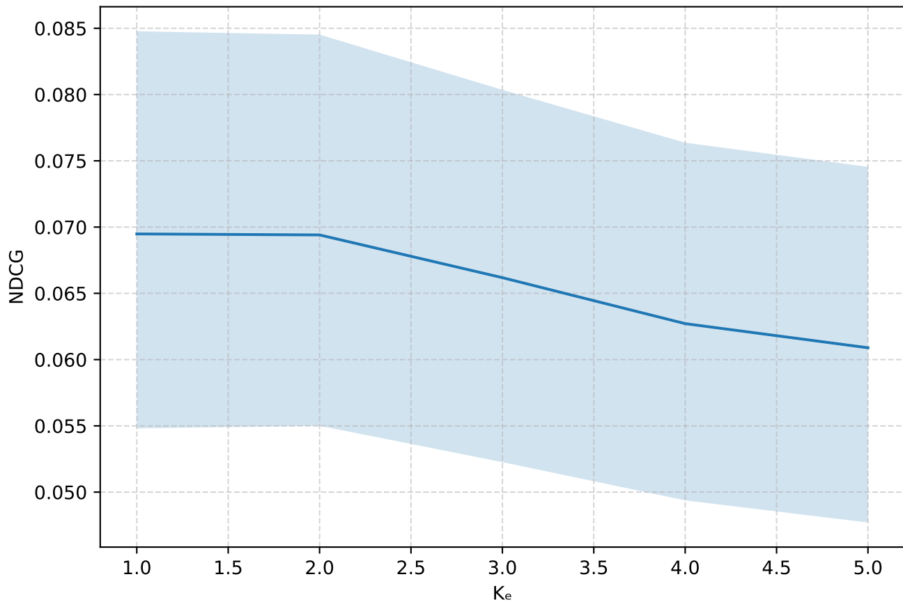
NDCG with 95% CI — ACCENT
