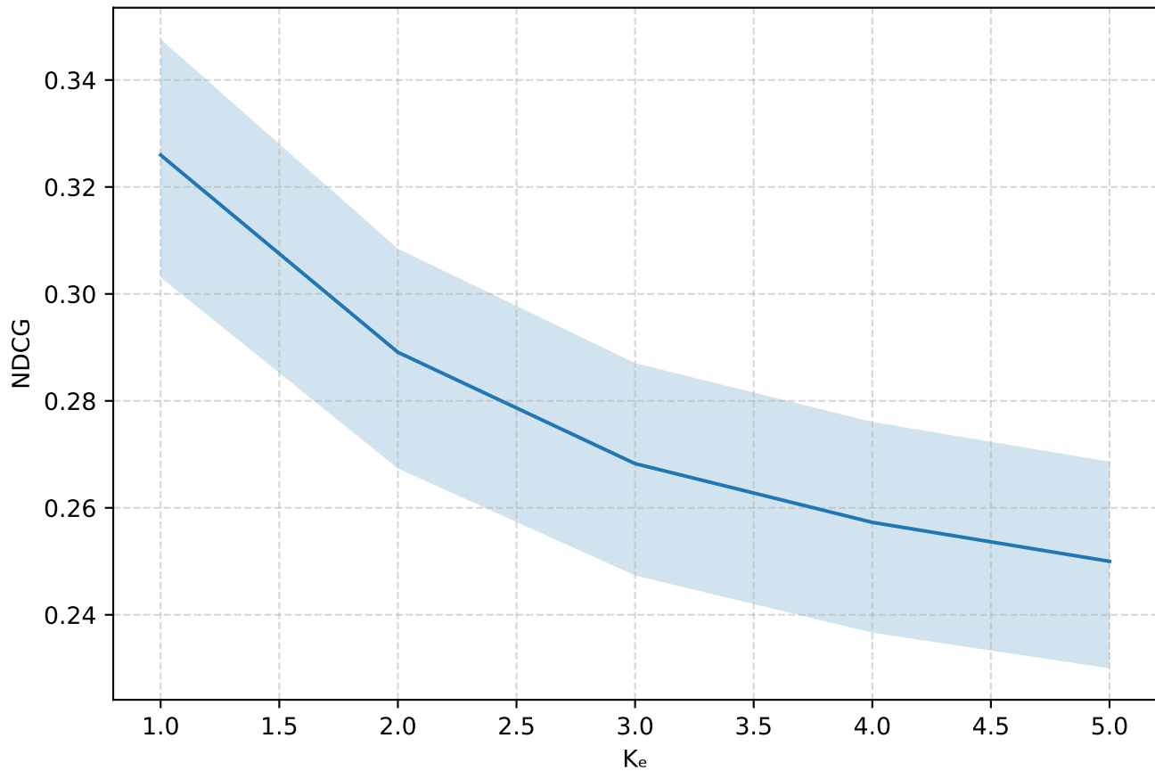
NDCG with 95% CI — COSINE
