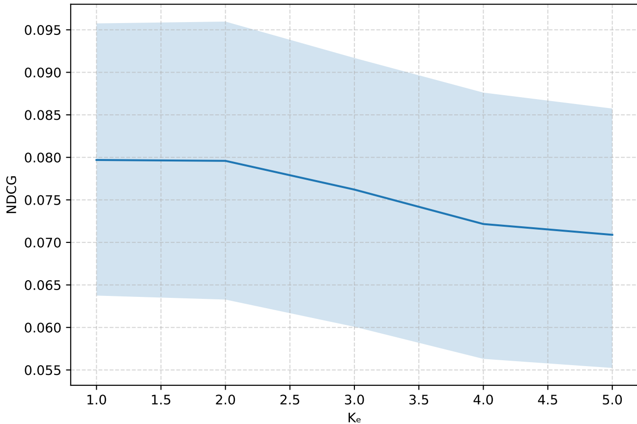
NDCG with 95% CI — LXR
