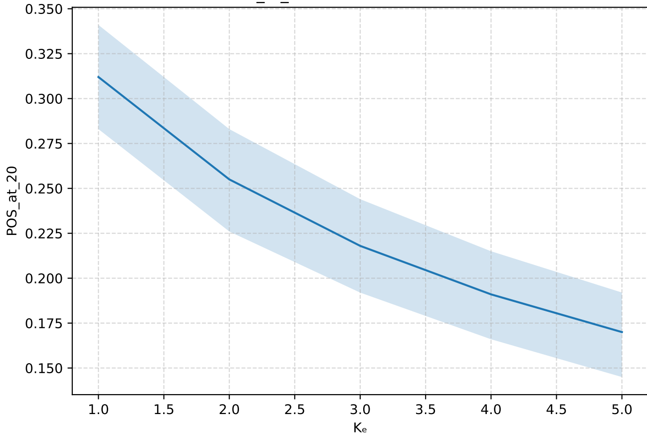
POS_at_20 with 95% CI — COSINE
