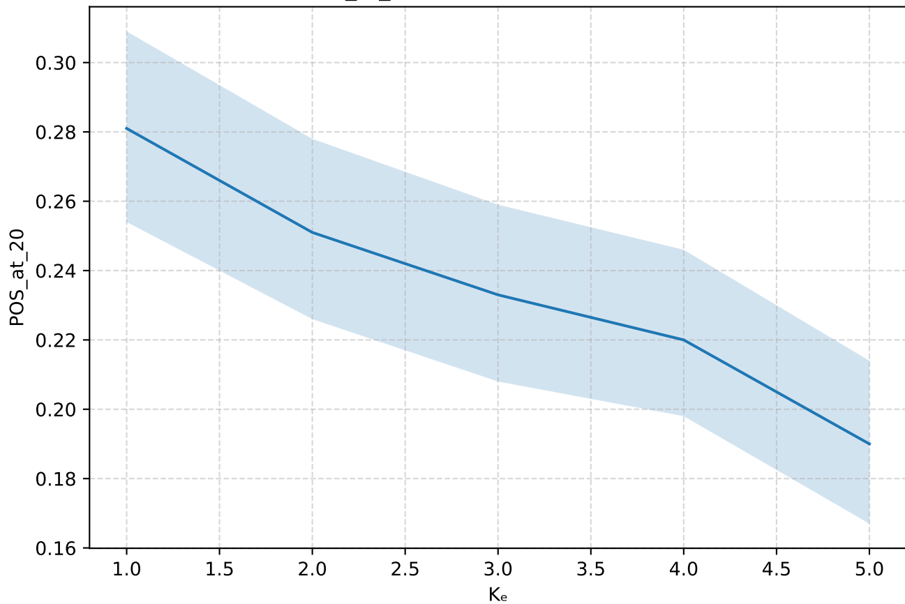
POS_at_20 with 95% CI — JACCARD
