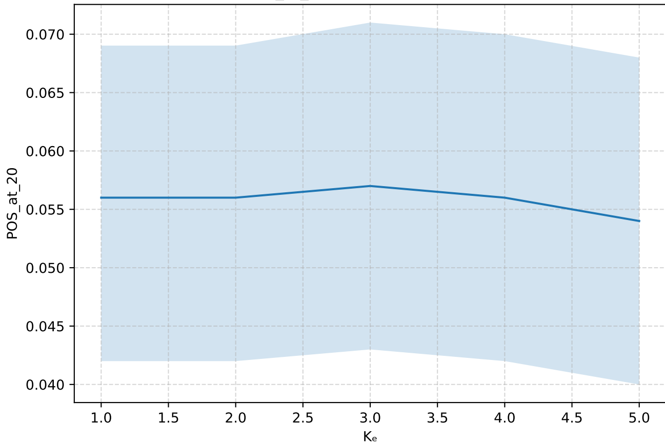
POS_at_20 with 95% CI — LIME
