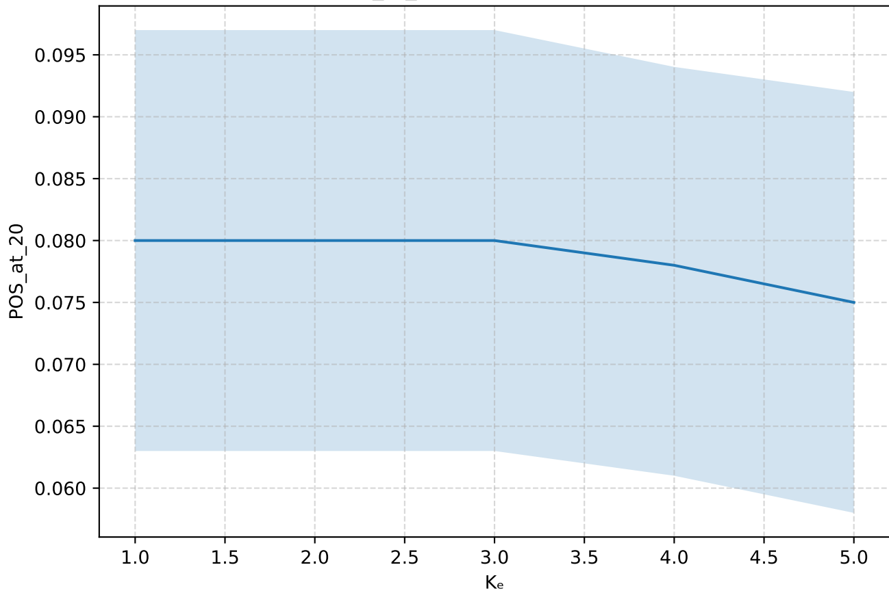
POS_at_20 with 95% CI — LXR
