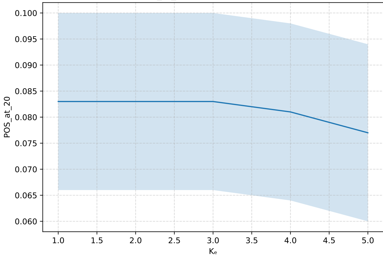
POS_at_20 with 95% CI — SHAP
