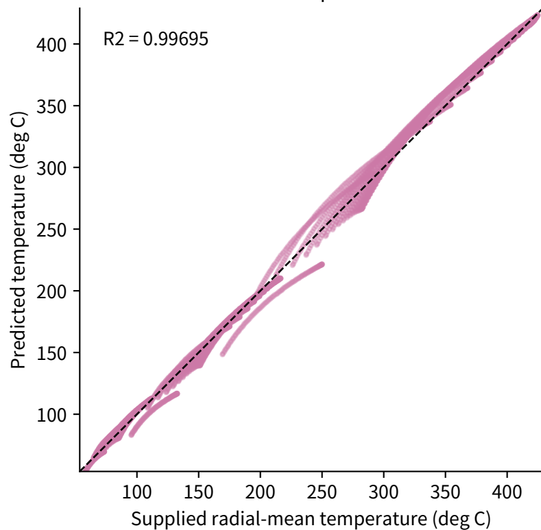
ASL-DeepONet
