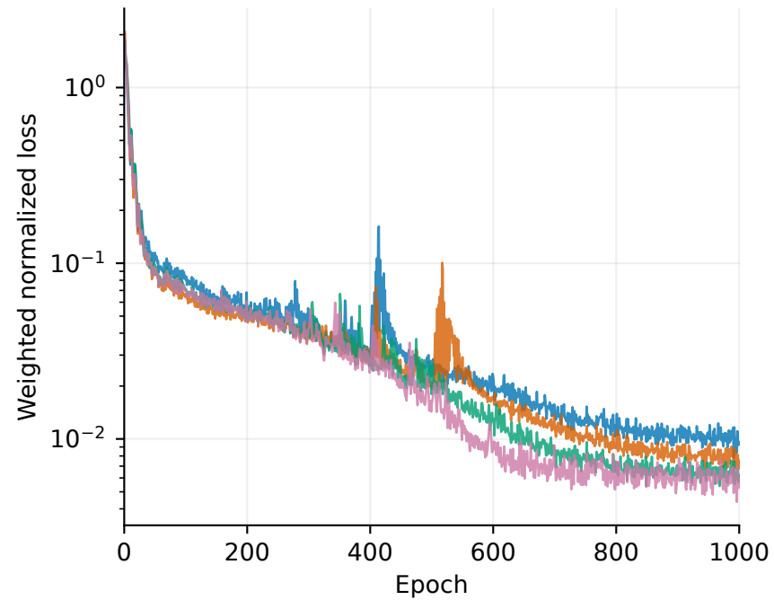
Training objective
