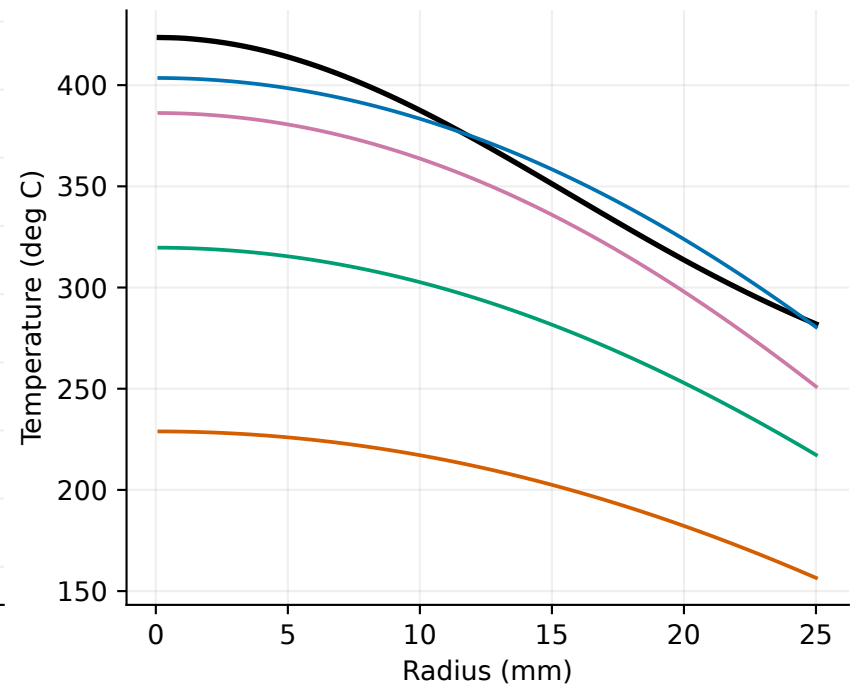
634 W, 120 s
