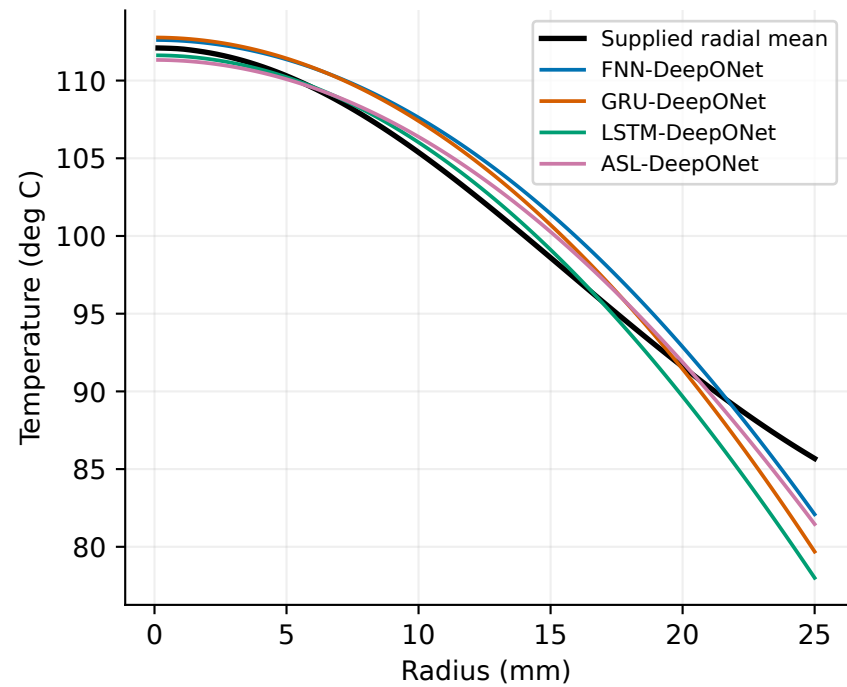
169 W, 80 s
