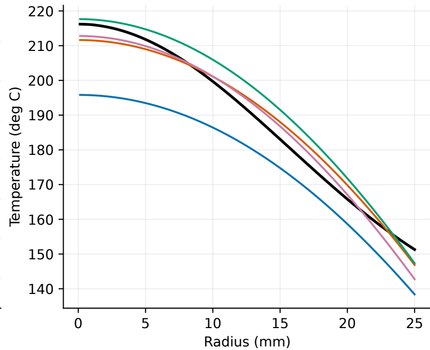
339 W, 100 s
