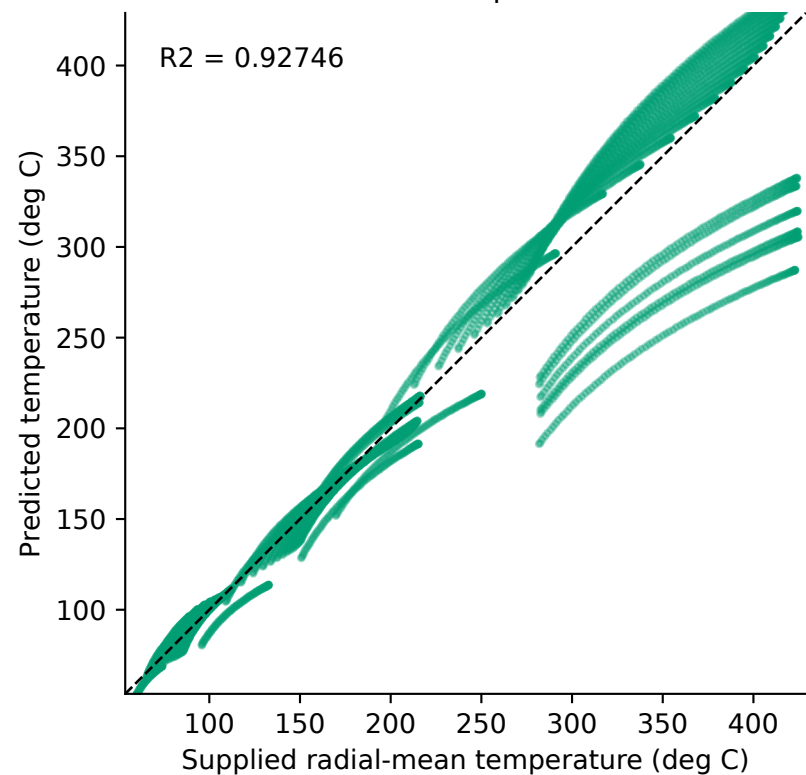
LSTM-DeepONet
