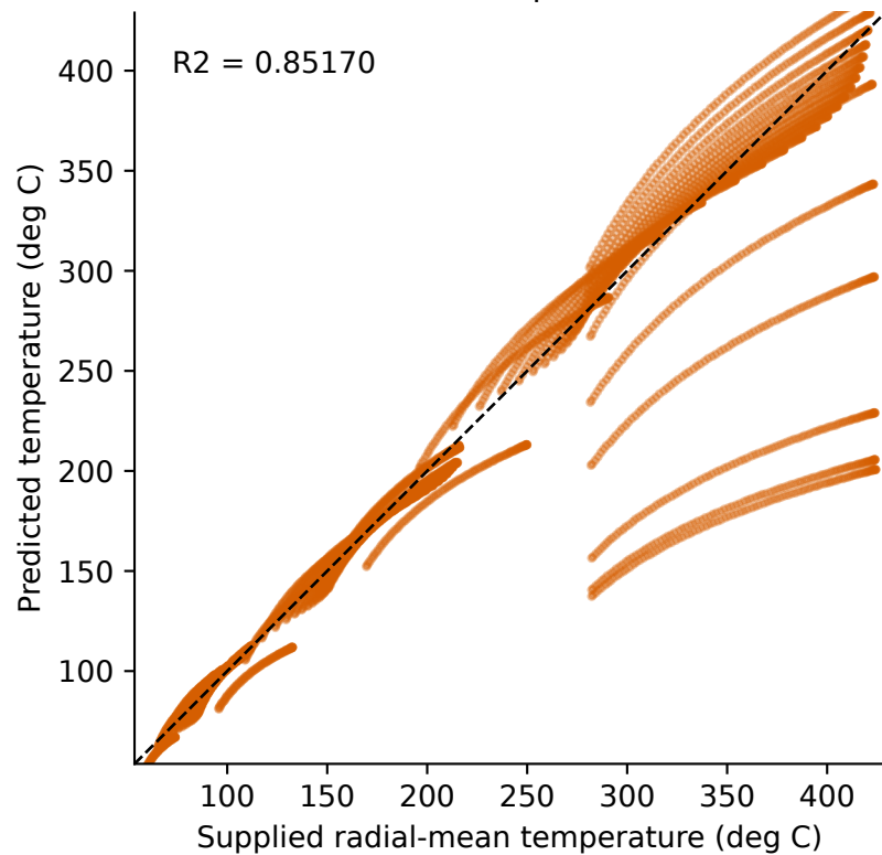
ASL-DeepONet
