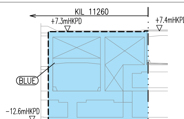
SECTION C NOT TO SCALE
