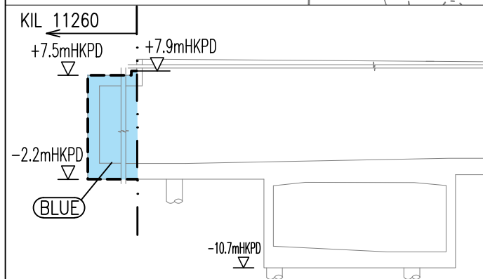
SECTION A NOT TO SCALE
