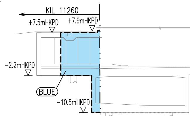
SECTION B NOT TO SCALE
