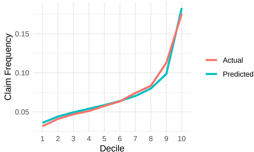
Decile Plot: Actual vs Predicted (Training Set)
