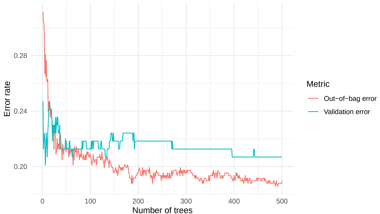
Figure 1: Random forest out-of-bag error versus validation error.
