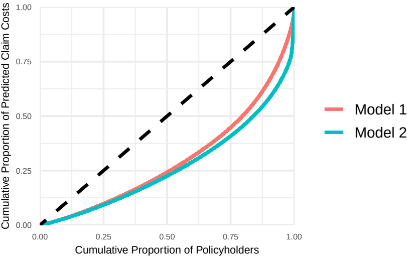
Gini Curve Comparison for Two Models
