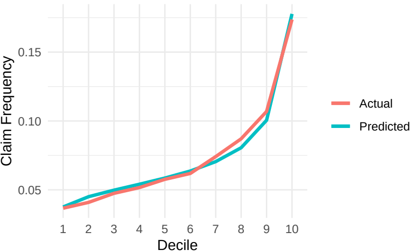
Decile Plot: Actual vs Predicted (Training Set)
