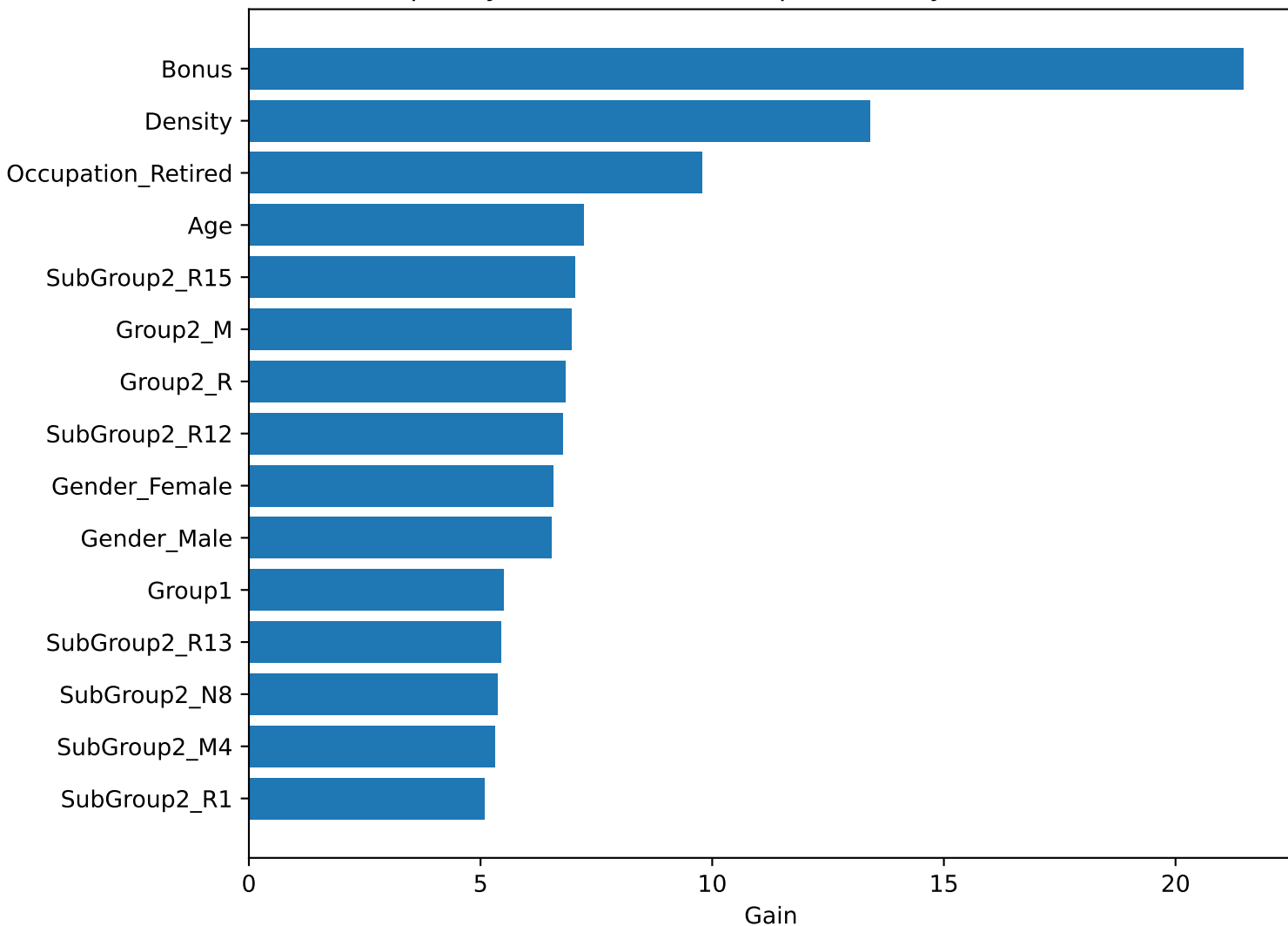
Frequency model: XGBoost importance by encoded feature
