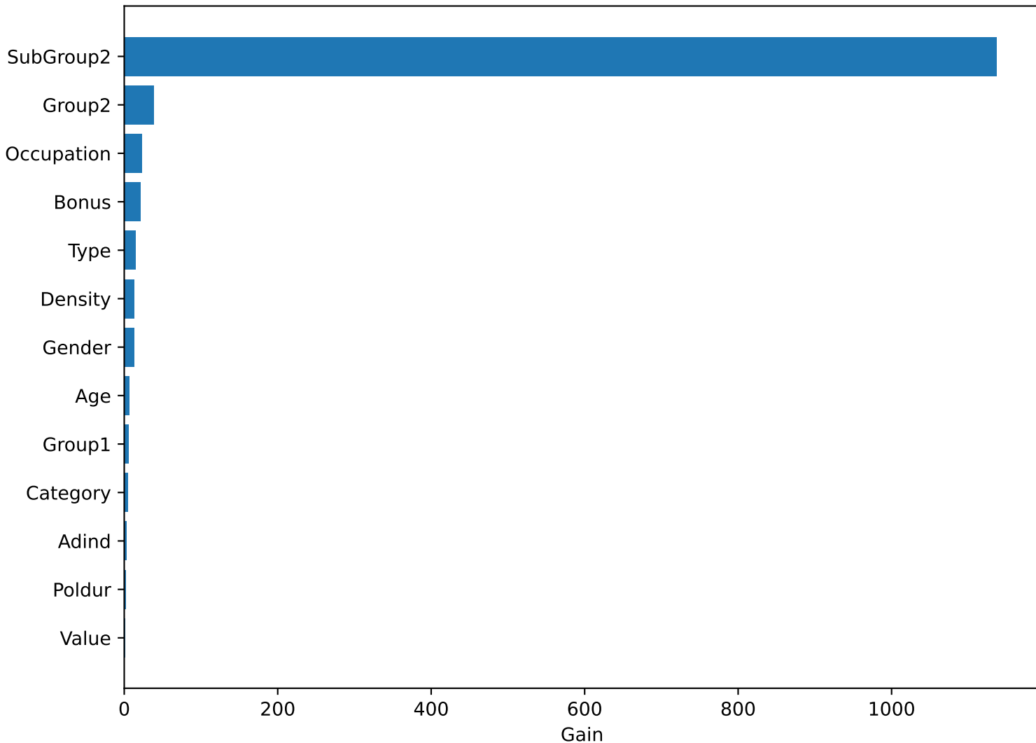
Frequency model: grouped XGBoost importance
