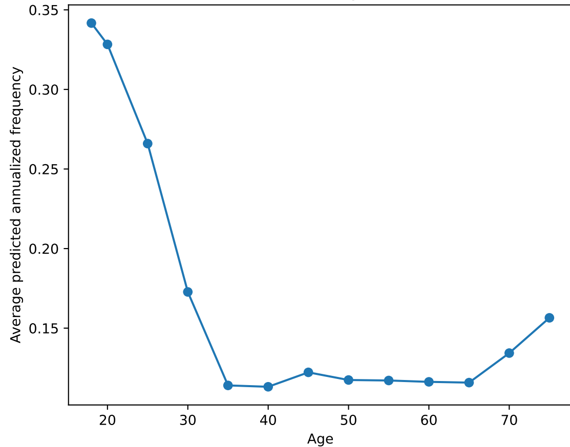
PDP for Age
