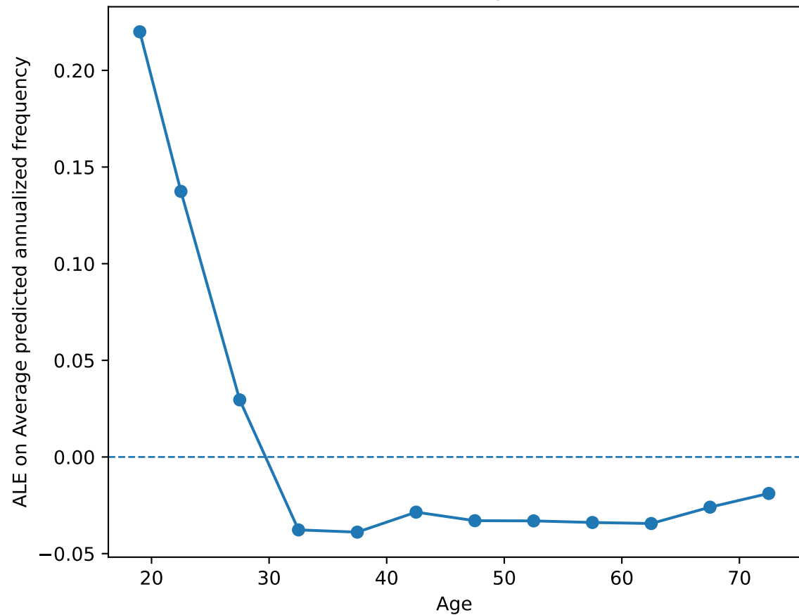
ALE for Age
