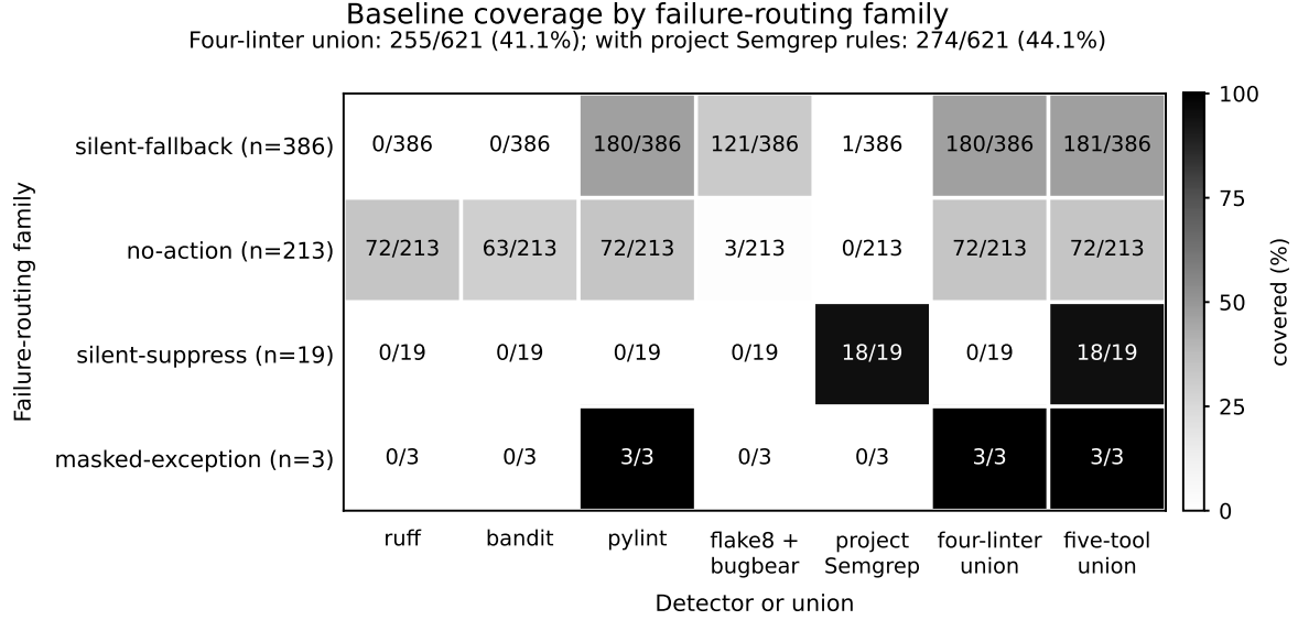
Figure 1: Coverage of the 621 pinned findings by rule family and detector. Each cell gives covered findings / family total; shading encodes the coverage share. The four-linter union covers 255/621 findings; adding the project’s supplementary semgrep rules covers 274/621. silent-suppress is the one family where the four linters, ruff ’s full 969-rule set and pylint ’s full default set all return zero coverage.
