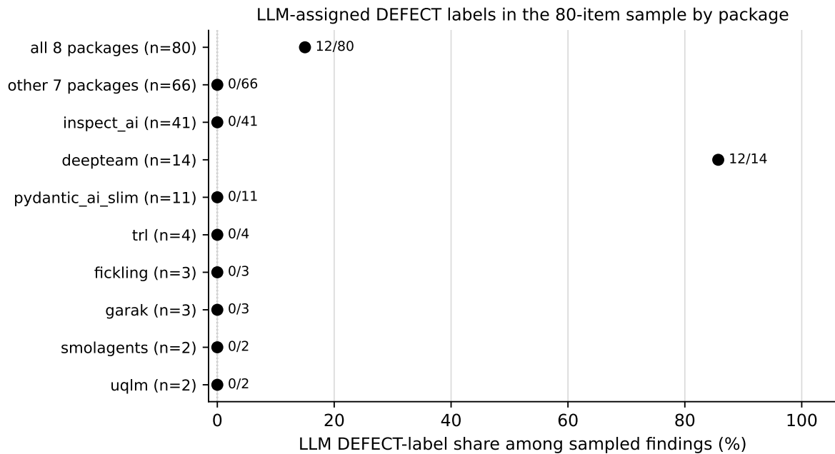
Figure 2: Share of sampled records assigned the LLM DEFECT label by package. The plotted shares and counts describe the 80-item sample; they are not package-level defect-rate estimates.
