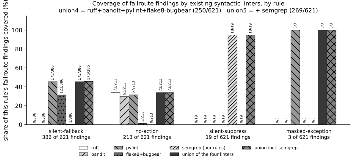
Figure 1: Per-rule coverage by tool, including the four-linter union and the five-tool union. silent-suppress is the one rule where the selected rule sets, ruff ’s full 969-rule set and pylint ’s full default set all return zero coverage.
