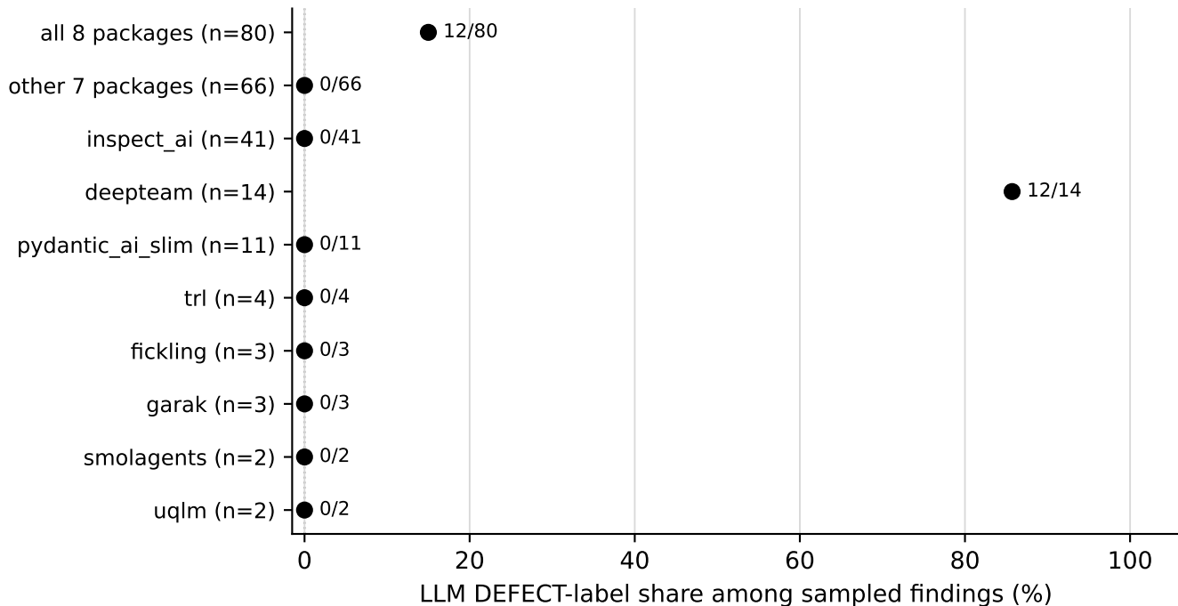
LLM-assigned DEFECT labels in the 80-item sample by package
