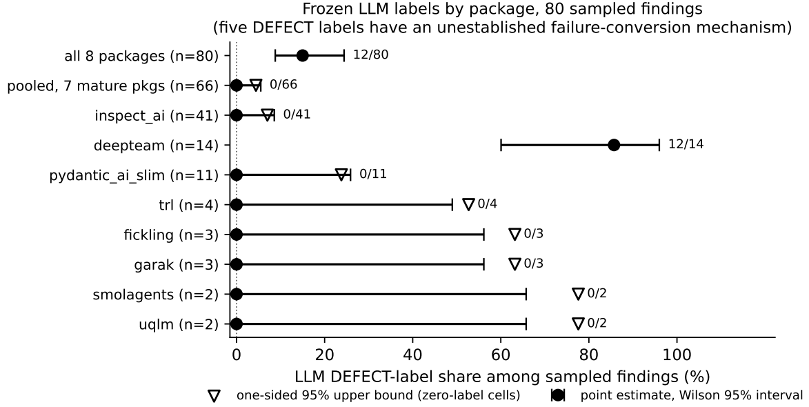
Figure 2: LLM DEFECT-label share per package with Wilson 95% intervals. Zero-label cells are drawn as exact one-sided 95% Clopper–Pearson upper bounds (triangles). The visual point is the spread, not the ordering.
