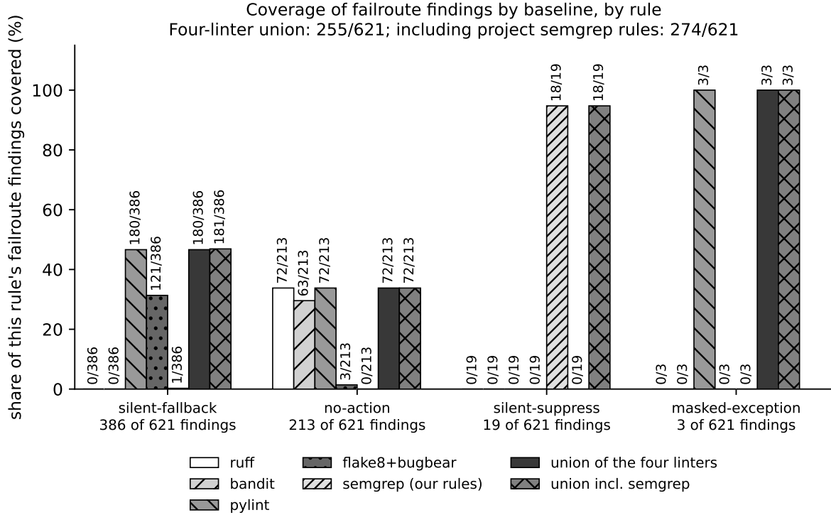
Figure 1: Per-rule coverage by tool, including the four-linter union and the five-tool union. silent-suppress is the one rule where the selected rule sets, ruff ’s full 969-rule set and pylint ’s full default set all return zero coverage.
