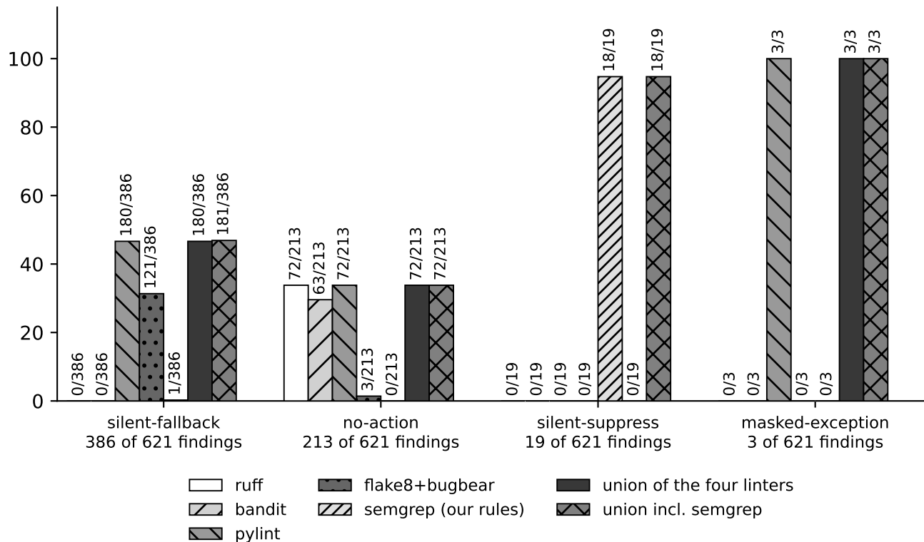
Coverage of failroute findings by baseline, by rule Four-linter union: 255/621; including project semgrep rules: 274/621
