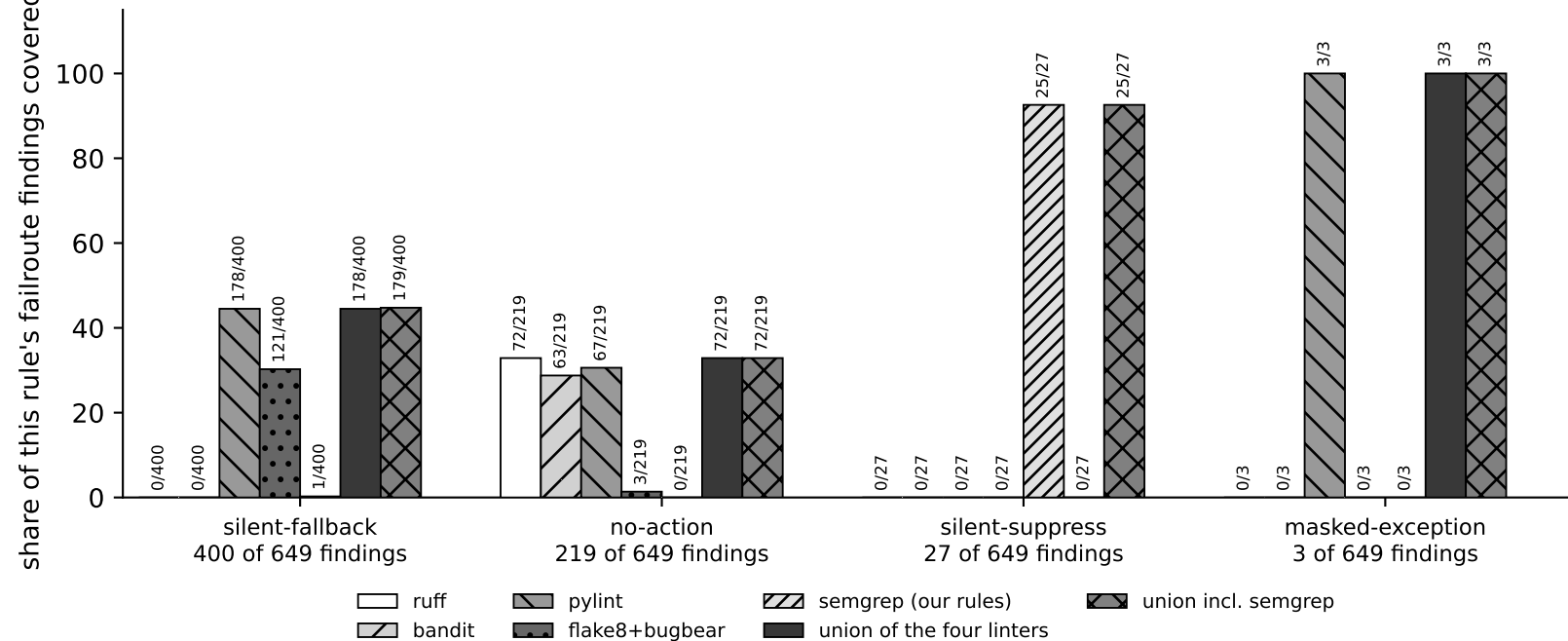
Coverage of failroute findings by existing syntactic linters, by rule union4 = ruff+bandit+pylint+flake8-bugbear (253/649) union5 = + semgrep (279/649)
