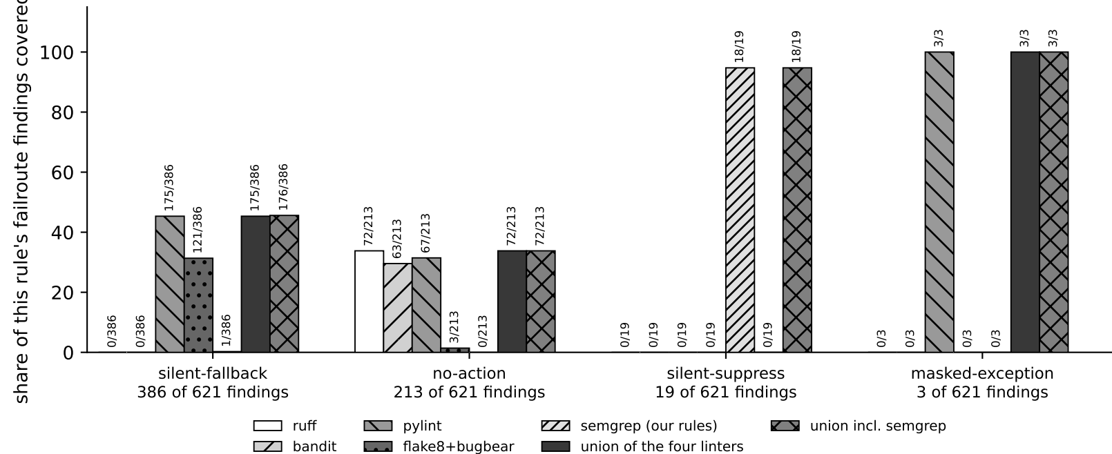
Coverage of failroute findings by existing syntactic linters, by rule union4 = ruff+bandit+pylint+flake8-bugbear (250/621) union5 = + semgrep (269/621)
