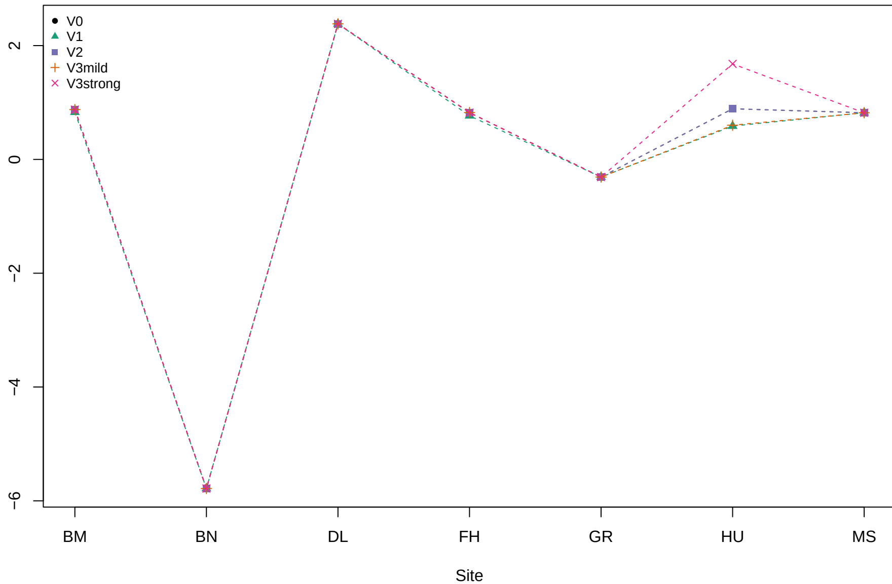
Temp driver share, high bracket, EOC 2098
