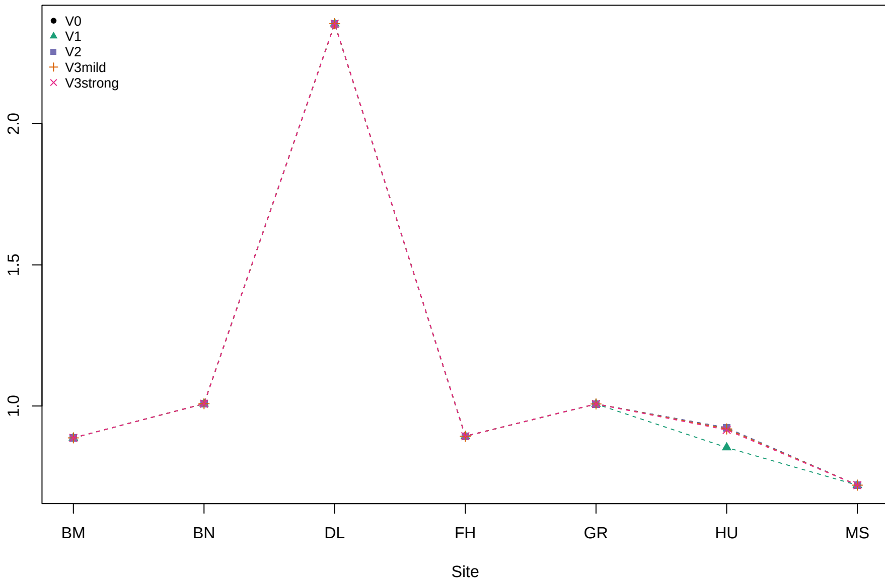
Temp driver share, low bracket, EOC 2098
