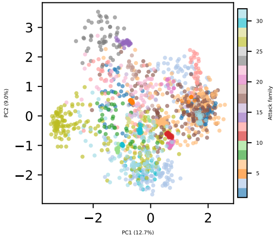
PCA of Layer-15 Activations
