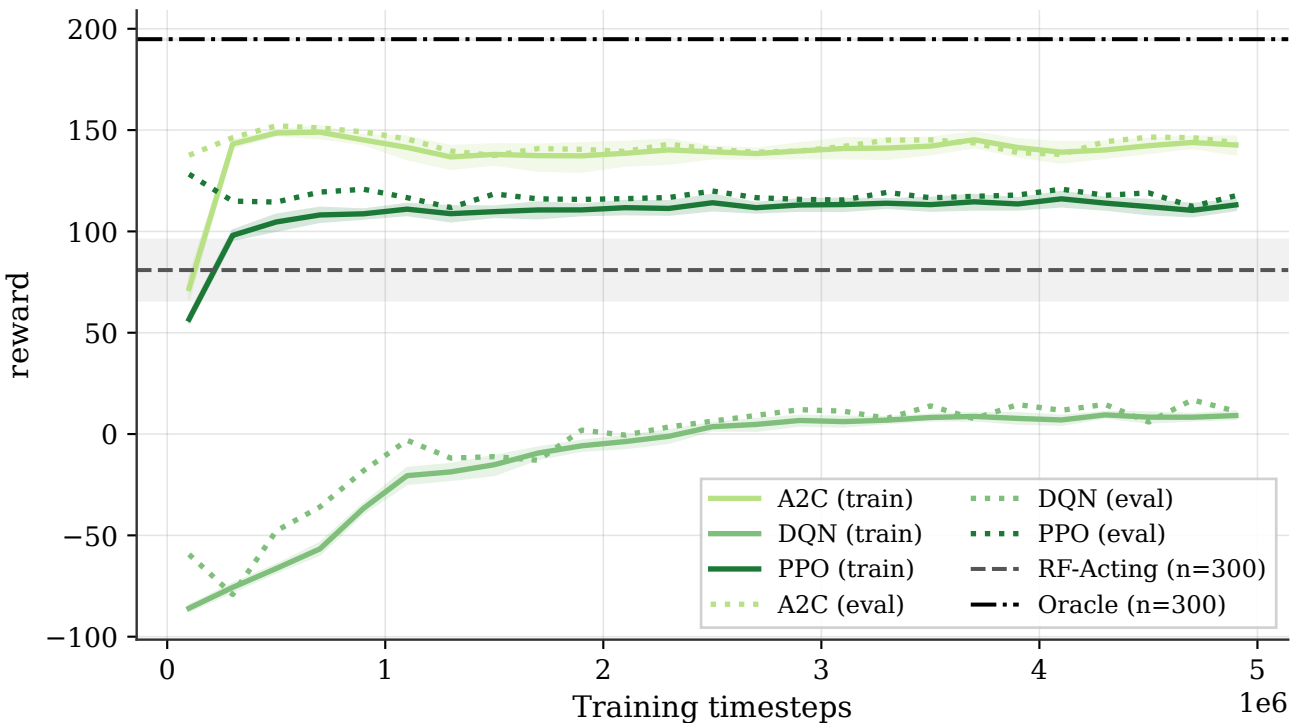
Mean episodic reward over training (A2C/DQN/PPO, 10 seeds per algorithm; 25 time bins; bands = 95 % bootstrap CI across seeds)
