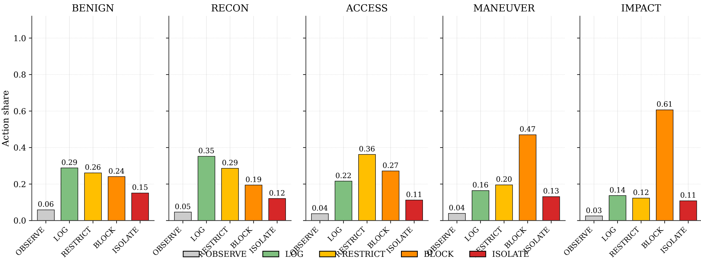
PPO per-stage action distribution of the converged policy
