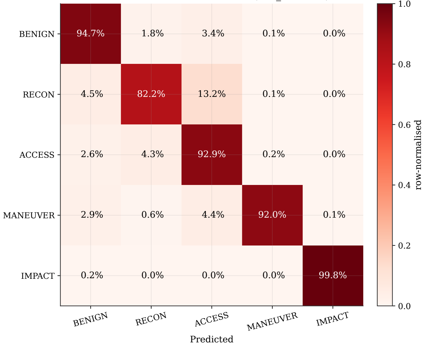
Tuned RandomForest confusion (test_balanced)
