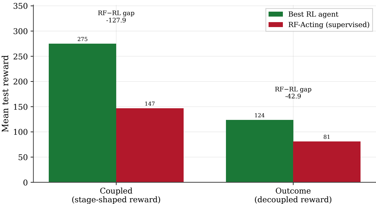
Reward design controls RF-Acting's apparent advantage
