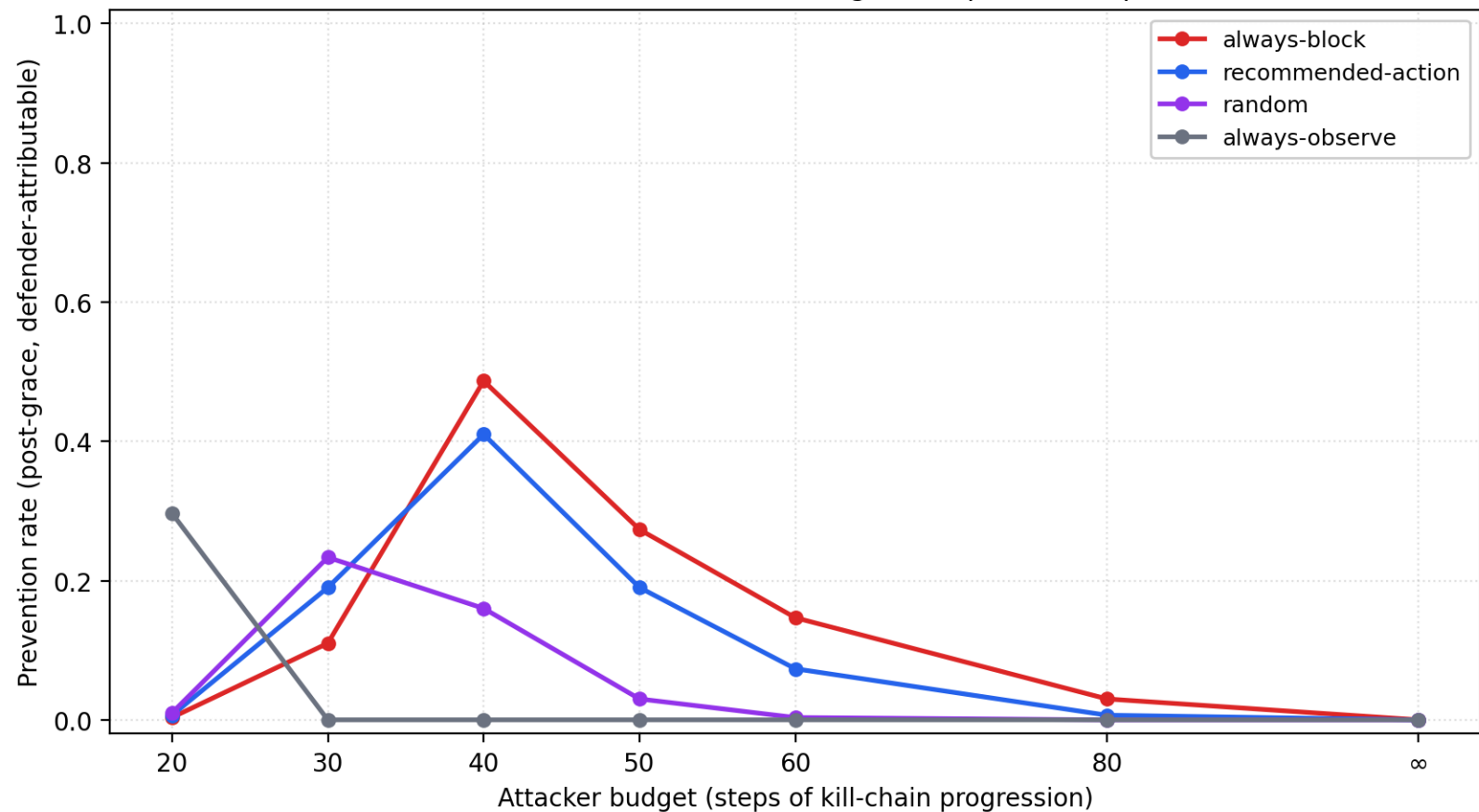
F16 — Prevention vs attacker budget (the prevention pivot)
