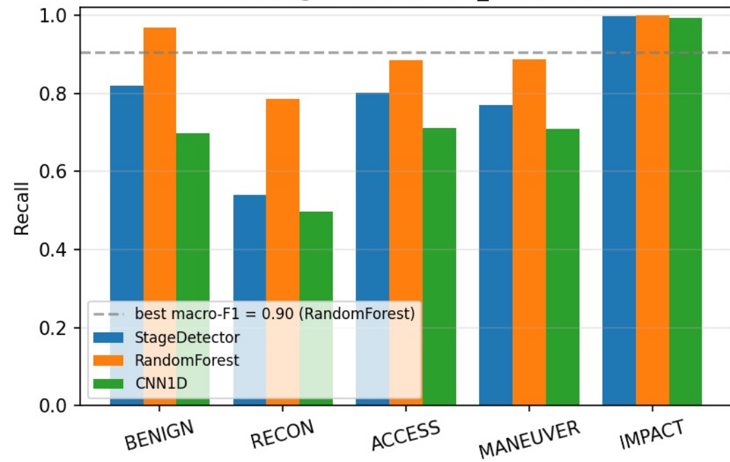
Per-stage recall on test_balanced
