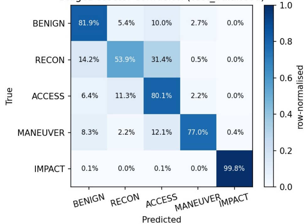
StageDetector confusion (test_balanced)
