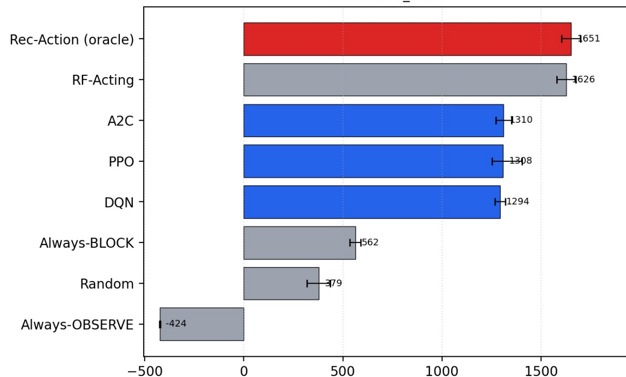
VulnerabilityScan
