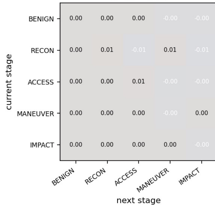
LSTM – Truth
