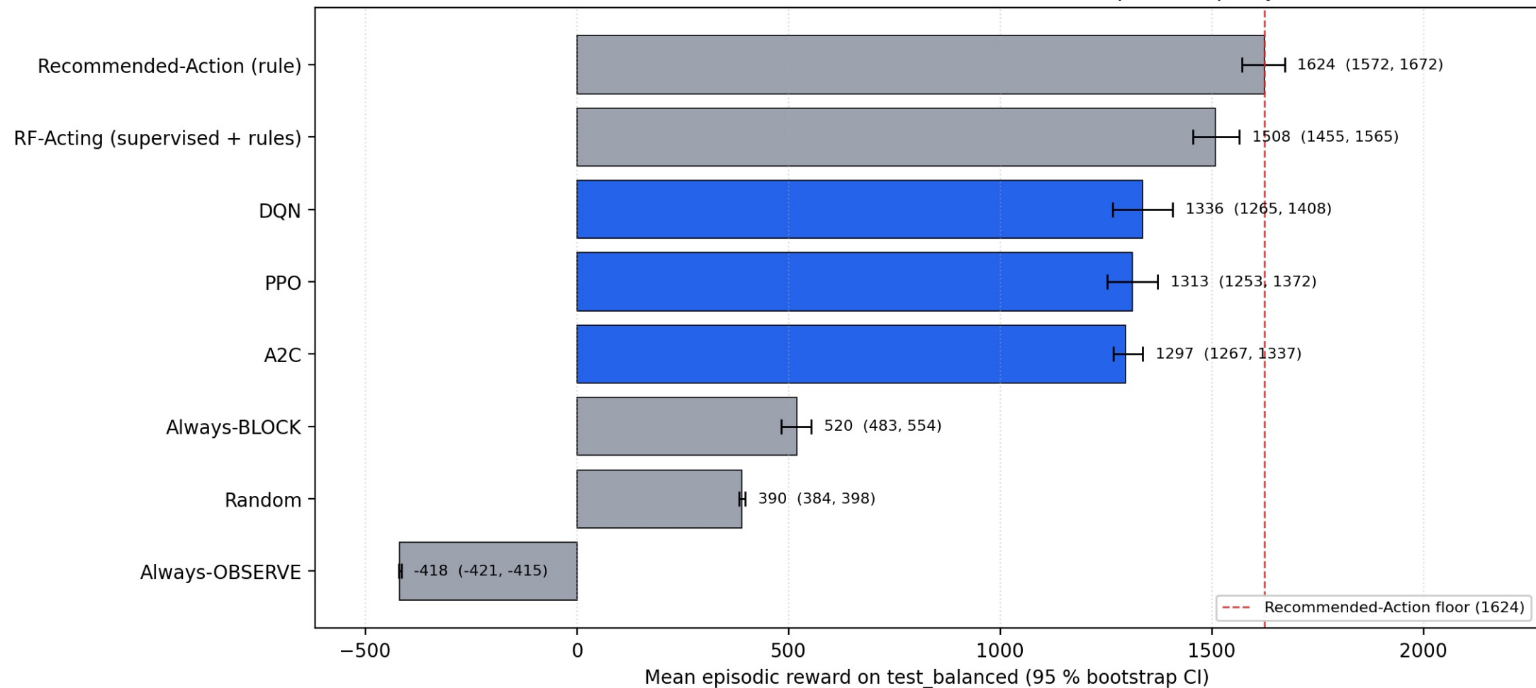
F8 — RL vs Non-RL Baselines (n=150 deterministic episodes / policy)
