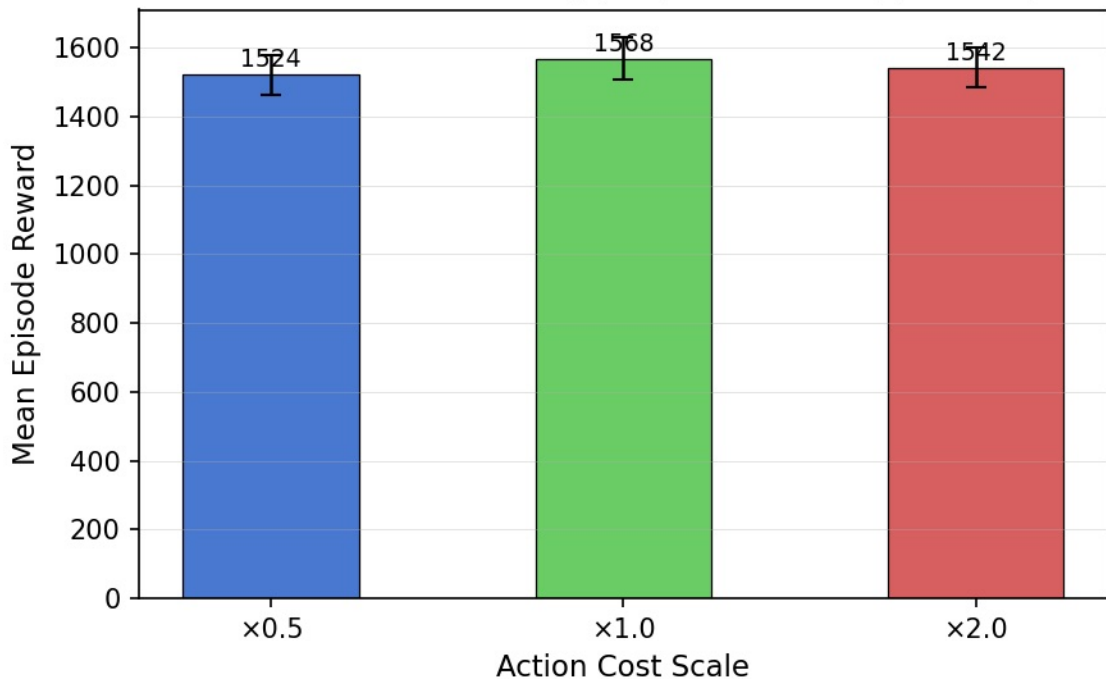
Action-Cost Scale Sensitivity (PPO, 3 seeds \times 30 ep, last 10%)
