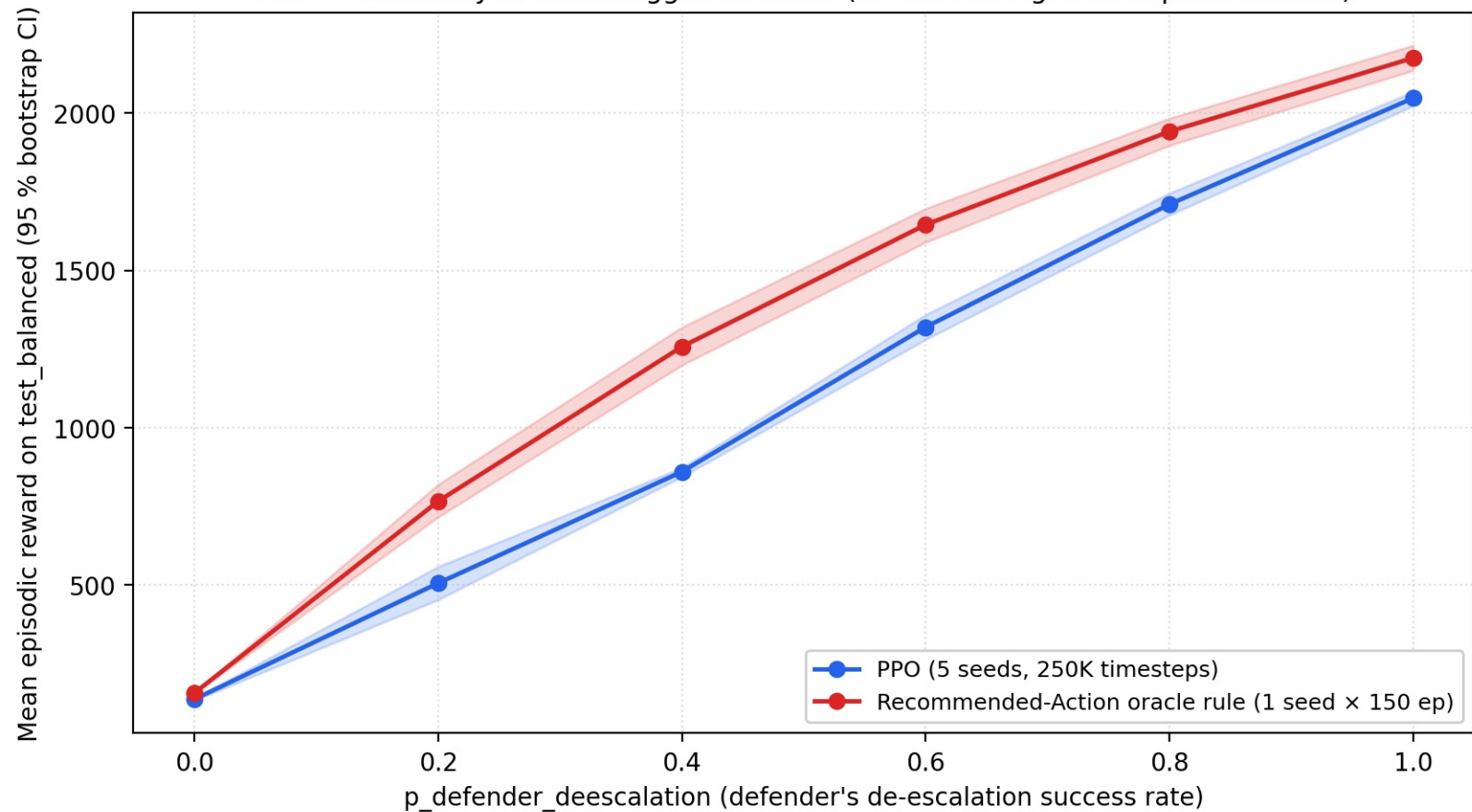
F10 — Sensitivity to attack aggressiveness (IoTWarden Fig. 6 re-implementation)
