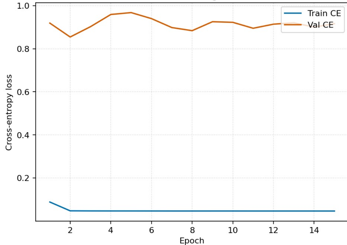
LSTM Red Team — training / validation loss
